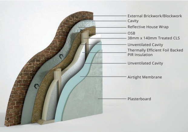
Wall Option 3 U-value - 0.19 W/m²k Overall Width - 314mm
