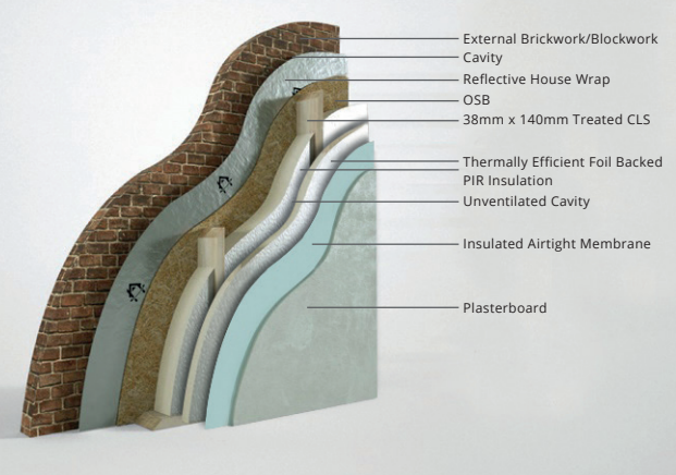
Wall Option 1 U-value - 0.16 W/m²k Overall Width - 339mm
