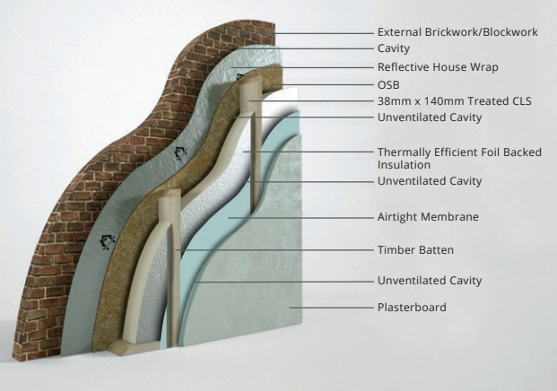
Wall Option 2 U-value - 0.17 W/m²k Overall Width - 339mm
